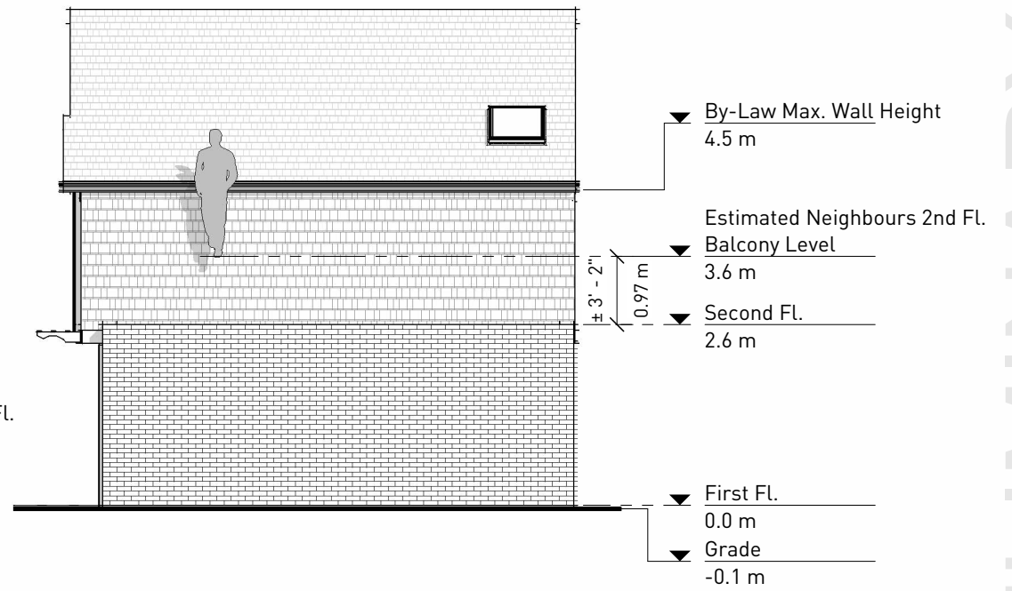
1 Proposed Right Elevation 1/8" = 1'-0"
