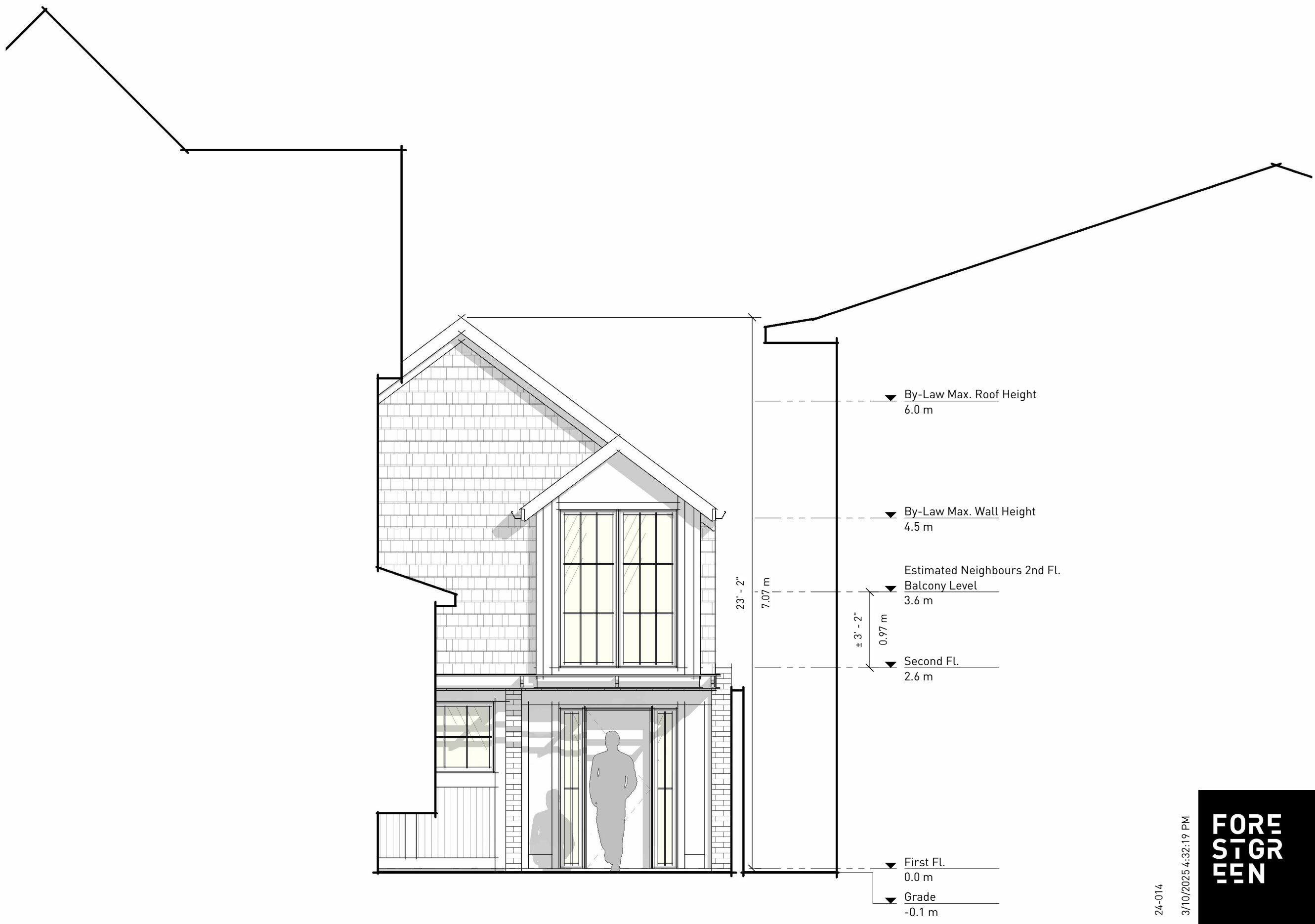
1 Proposed Front Elevation From Street 1/4" = 1'-0"
